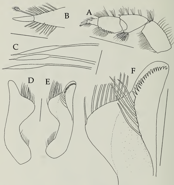
Fig. 7. Pseudopaguristes shidairai , new species; holotype male (CBM-ZC 6814), SL = 2.55 mm, Miyako Is., Okinawa. Left fourth pereopod: A, lateral; B, distal portion of dactyl, dorsal; C, ventral setae of carpus. Left first pleopod: D, external; E, internal; F distal portion, internal, enlarged. Scales equal 1 mm (A) and 0.2 mm (B-E).
